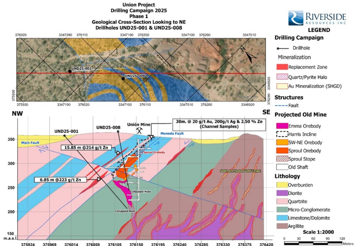
Figure 1: Cross section through the Union Mine area showing Phase 1 drill holes (including holes 1 and 8), interpreted mine workings/ore zones, and the location of the continuous channel sample along the Union Mine decline wall. The section illustrates the spatial relationship between the high-grade Au-Ag-Zn channel interval and nearby drill intercepts and provides geological context for potential follow-up targeting for both CRD and SHGD.
