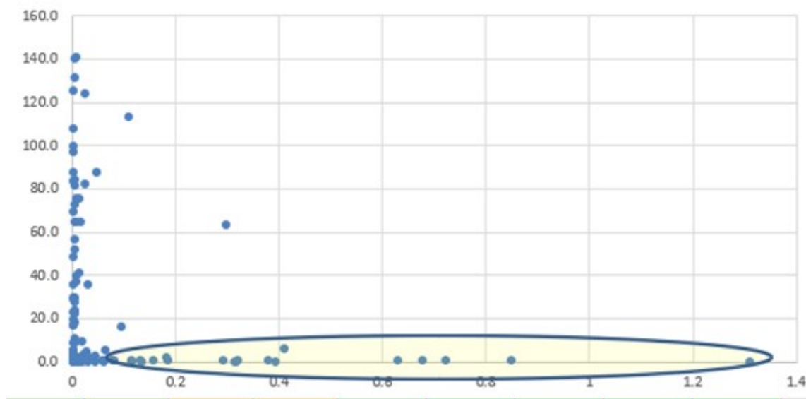
Figure 3: Gold with high Al + K + Na, meaning not with the dolomite and limestone for the sediment-hosted gold aspects like Nevada. Carlin geochemistry for the Luis Hill Hole 9.
